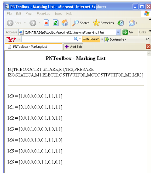
Fig. 4: List model
