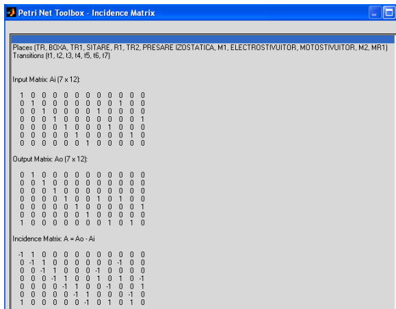
Fig. 2: Incidence matrix
